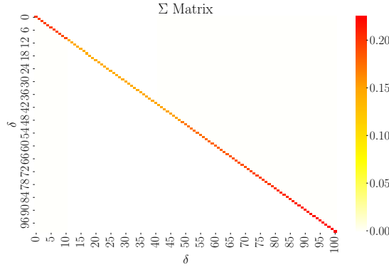
Figure 12: \Sigma matrix
